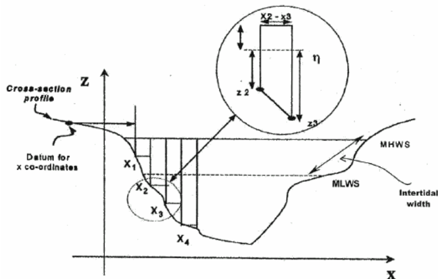
Figure 72. The method used in the 1D hybrid model for the calculation of the cross-sectional areas and intertidal width
