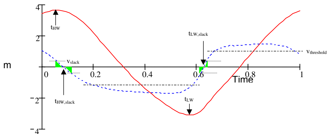
Figure 62. Change in slack duration during a flood and ebb tide
