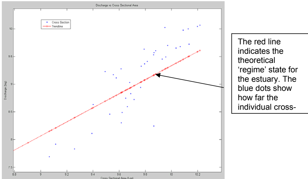
Figure 27. Regime fit (Cross-section area vs Maximum discharge)
